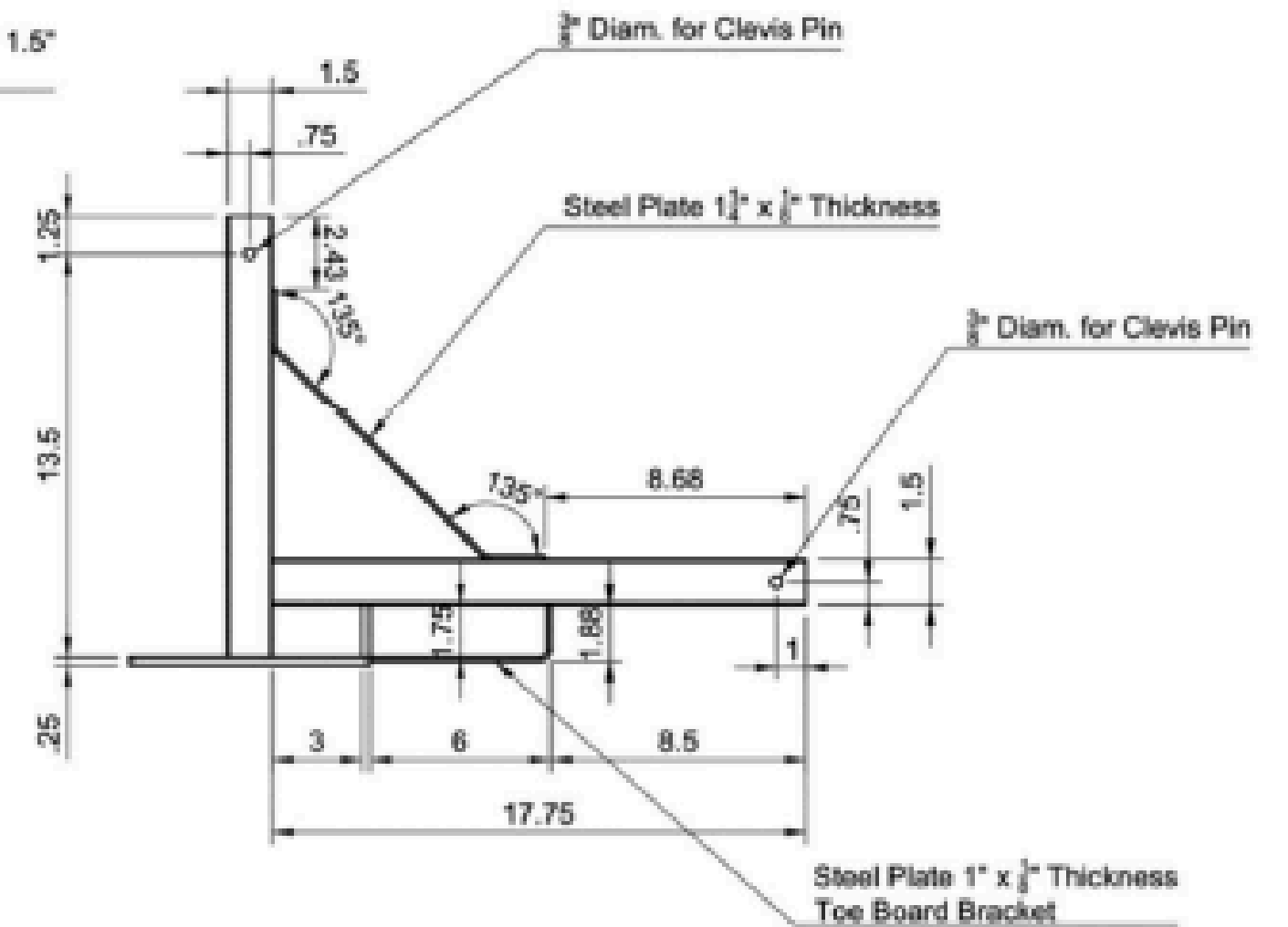
SIDE VIEW
